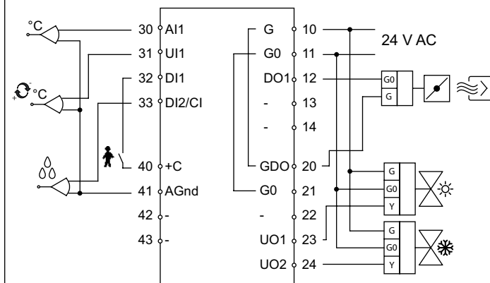
Figure 4. Connection diagram for RC-H
